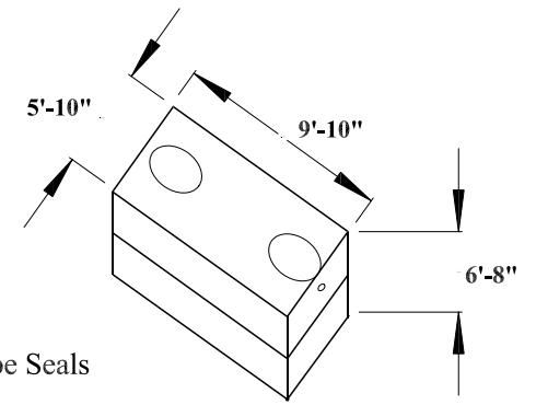
ASSEMBLED TANK
