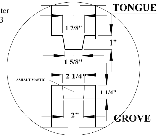
JOINT DETAIL
